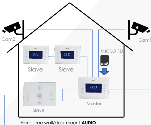
Handsfree wall/desk mount AUDIO Handset option.
