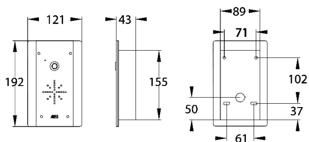
603-FB/FS CALL FLUSH PANEL
