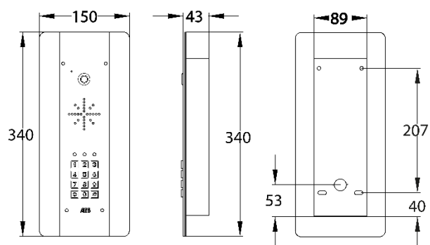
603-ABK/ASK CALL FLUSH PANEL
