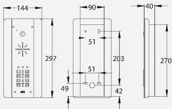
603-ABK/ASK CALL PANEL
